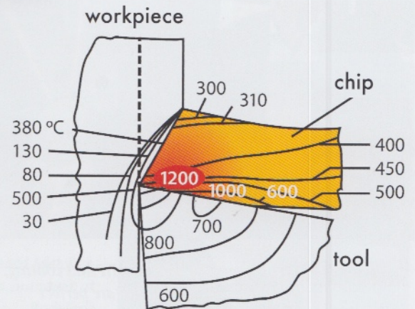
Titanium being a poor thermal conductor, the heat cannot be evacuated from the cutting zone via the chips; at temperatures of 1200°C the cutting tool can quickly sustain heat-related damage
